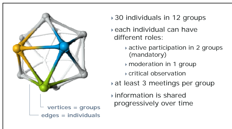
Figure 3: BrainSpace architecture
